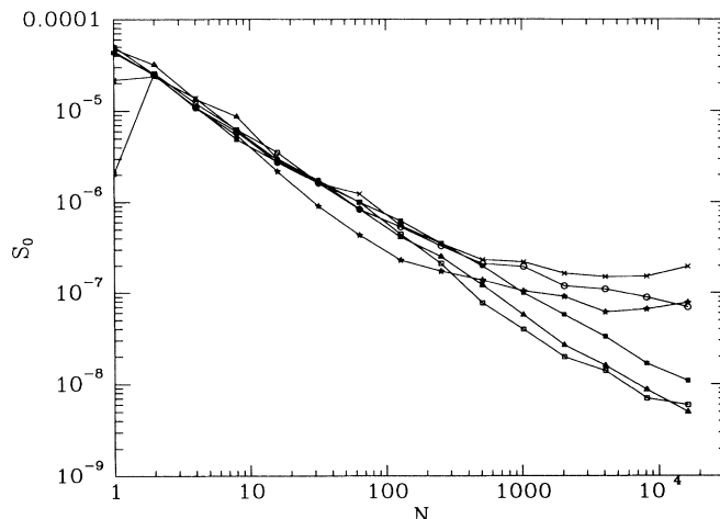
FIG. 2. Low frequency limit of the power spectrum, S_0 = \lim_{\omega \rightarrow 0} S(\omega) , as a function of the size of the array N , for \bar{g} = 0.2 , \Omega_{rf} = 0.8 , i_{rf} = 0.61 , i_{dc} = 0.124 and different values of \sigma . ( \Delta , \sigma = 0.1 ; \square , \sigma = 0.15 ; * , \sigma = 0.2 ; \circ , \sigma = 0.3 ; \times , \sigma = 0.4 ; \blacksquare , \sigma = 0.5 .)
